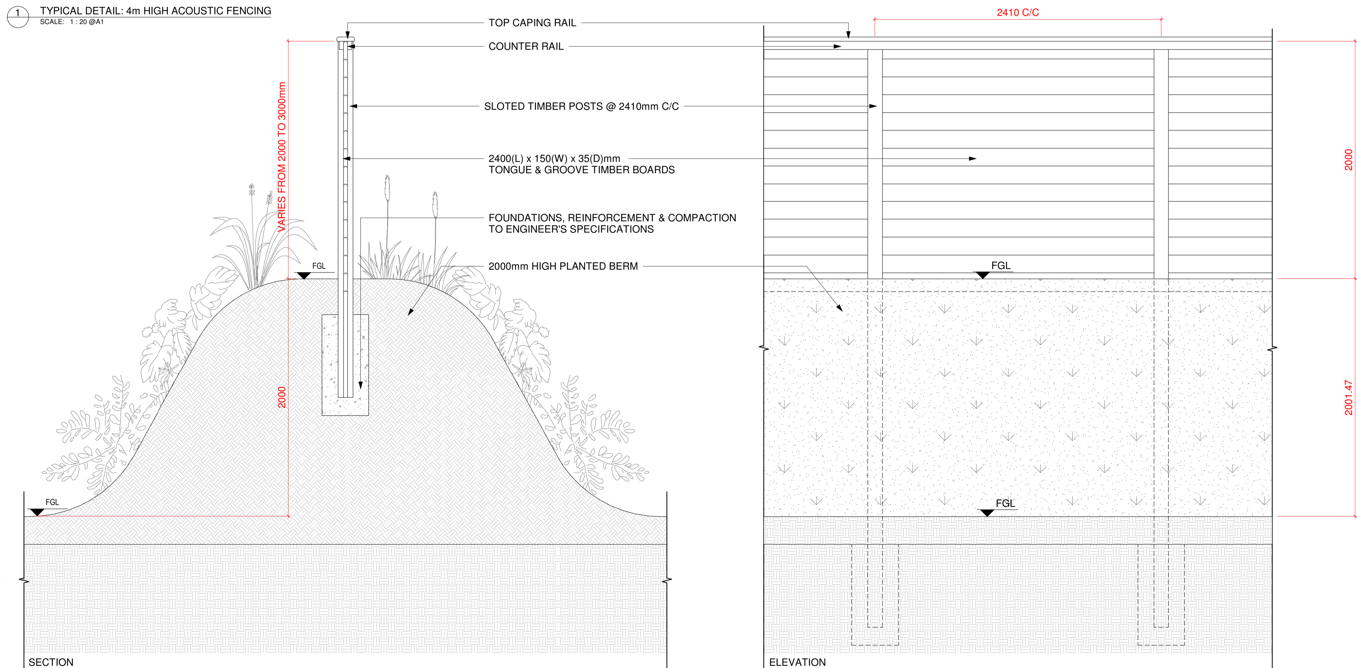
2 TYPICAL DETAIL: 2m HIGH ACOUSTIC FENCING ON 2m HIGH PLANTED BERM SCALE: 1:20 @A1
