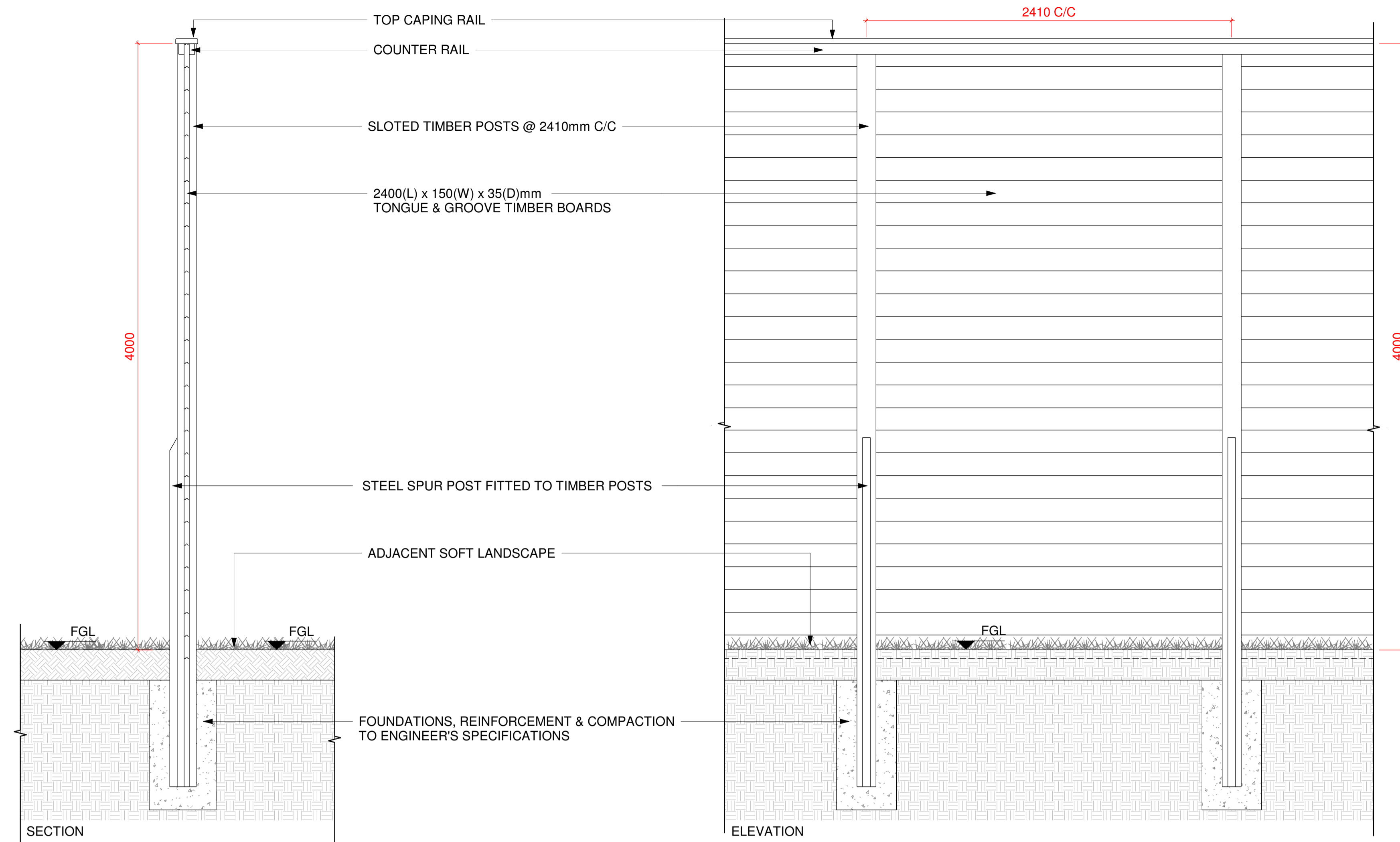
1 TYPICAL DETAIL: 4m HIGH ACOUSTIC FENCING SCALE: 1:20 @A1
